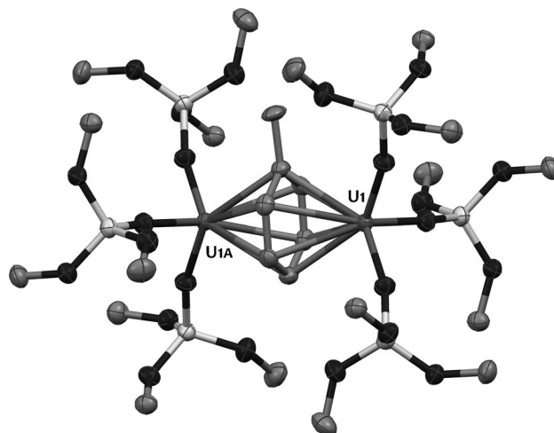
Figure 5. Ellipsoid plot (50% probability) for [ \{U(OSi(OtBu)_3)(\mu-\eta^6:\eta^6\text{-toluene})\}_2 ] ( 5 ) crystallized from hexane/toluene. Hydrogen atoms, siloxide methyl groups, and disorder were omitted for clarity.
